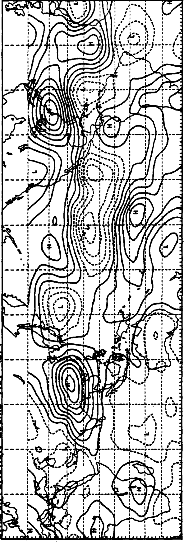
STREAM FUNCTION 200MB WIN 1974
